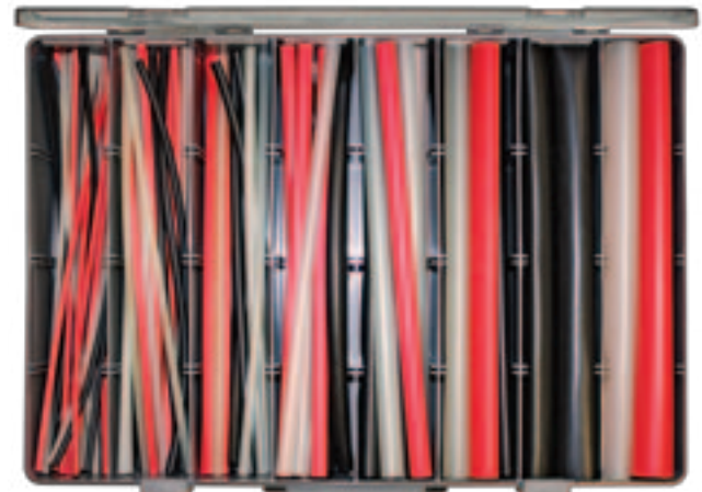
LARGE HEAT SHRINK KIT Part Number KIT-HS-LARGE Black, clear, and red adhesive lined dual wall shrink in 12" lengths. 1/8", 3/16", 1/4", 3/8", 1/2", 3/4" and 1" diameters. 134 pieces. Drawer satchel.
